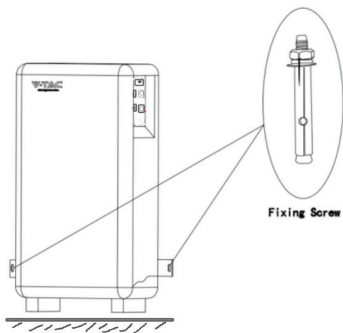
Fig.6-3 Fix the Battery to the Wall
