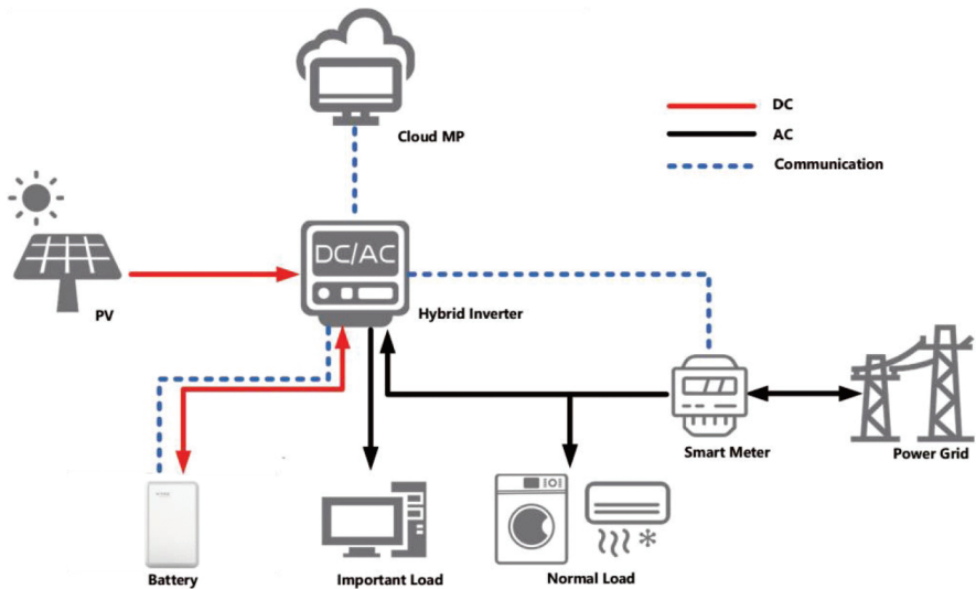
Fig. 3-1 Working Diagram of the Battery Pack
