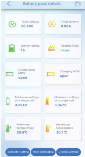
Figure 8: Battery pack details
