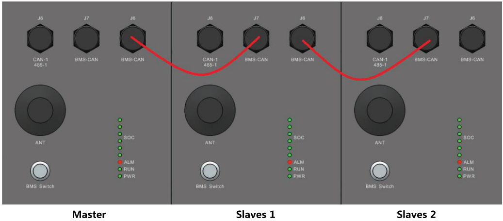
The Communication Port Definition
