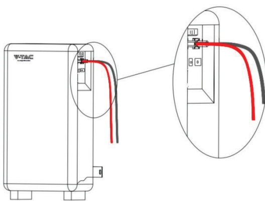
Fig.6-5 Communication Cable Connection Diagram
